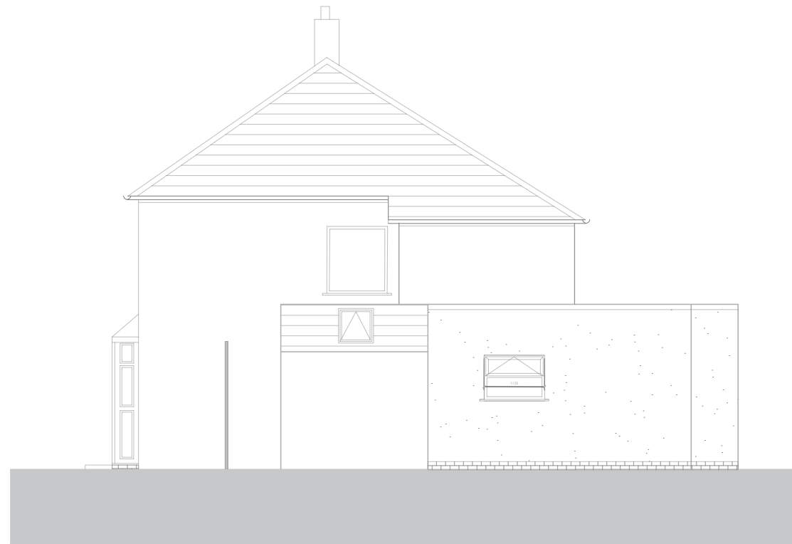
2 104 Proposed Side Elevation B 1:100@A3
