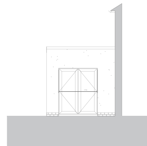
3 105 Proposed Side Elevation E 1:100@A3
