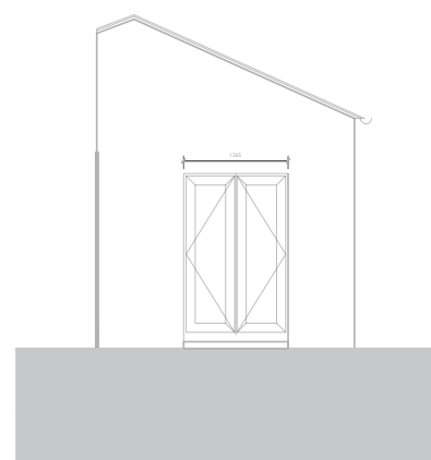
2 105 Proposed Rear Elevation D 1:100@A3
