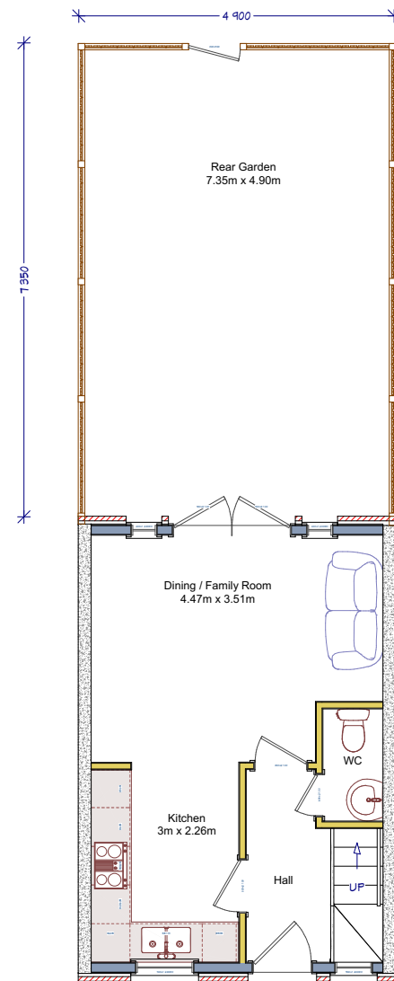
Existing Ground Floor Plan 1:50
