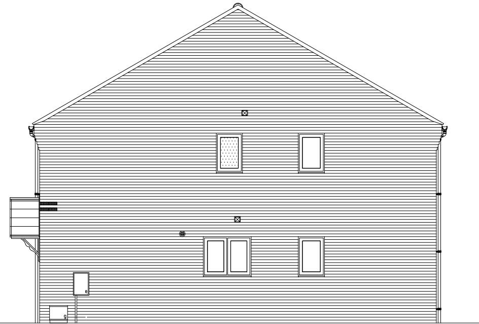
END ELEVATION - STANDARD
