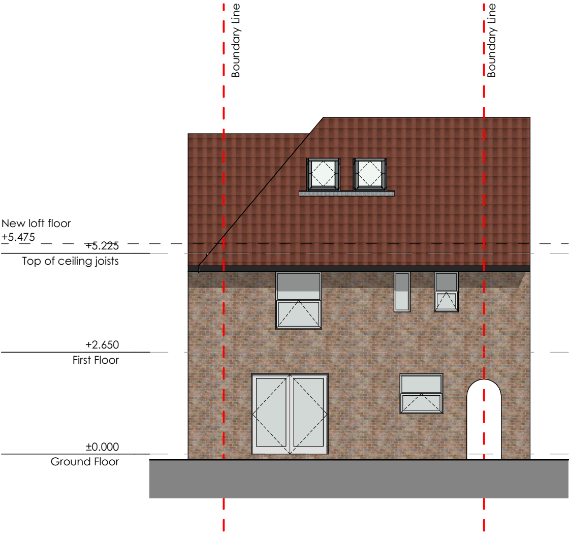
2 Proposed Rear Elevation 1:100
