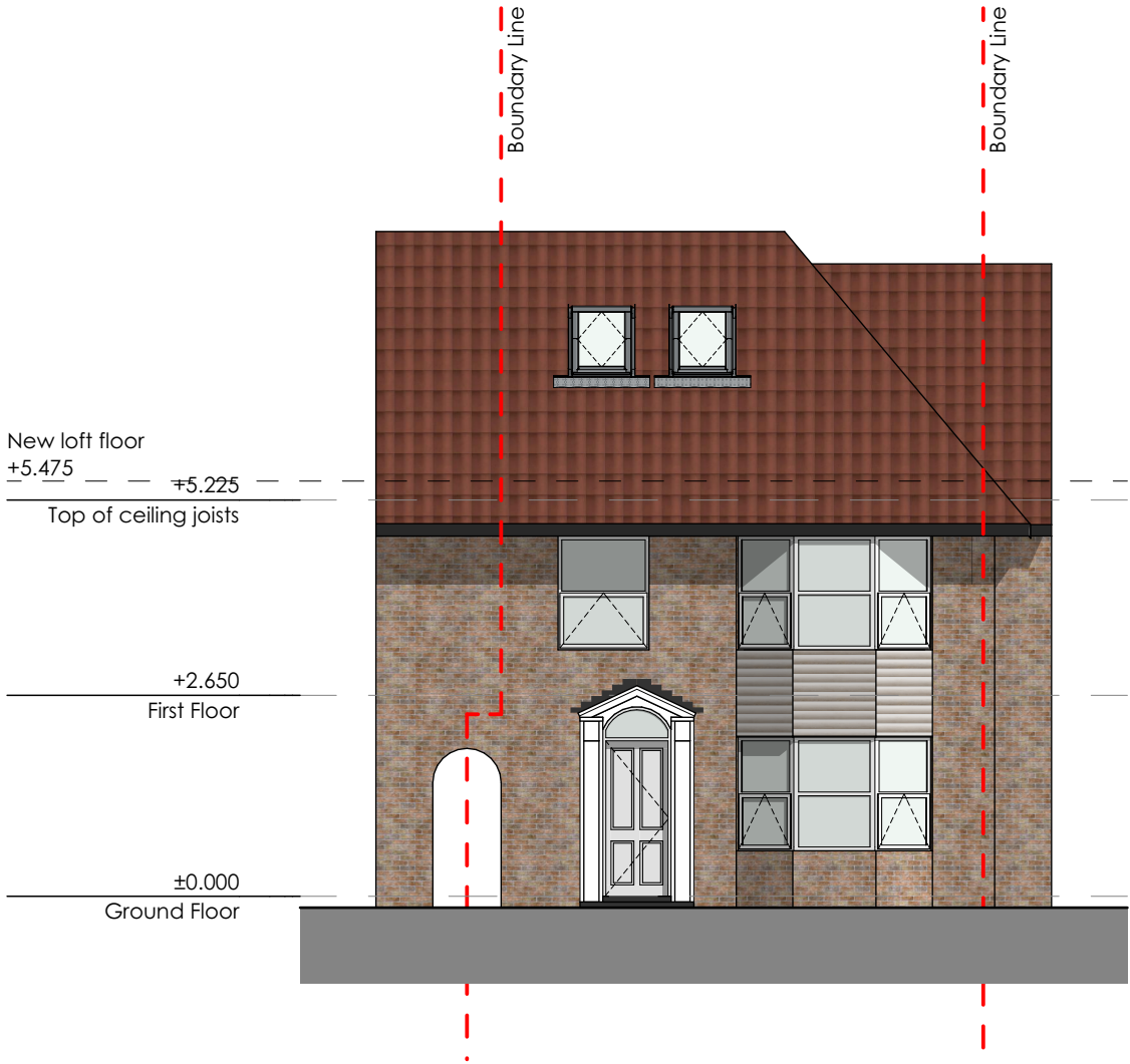
1 Proposed Front Elevation 1:100
