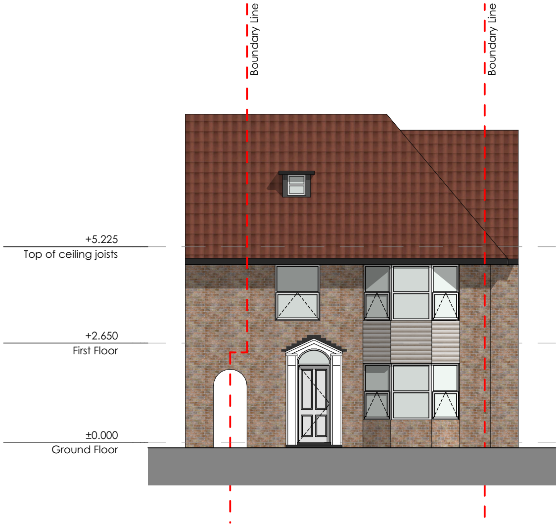
1 Existing Front Elevation 1:100
