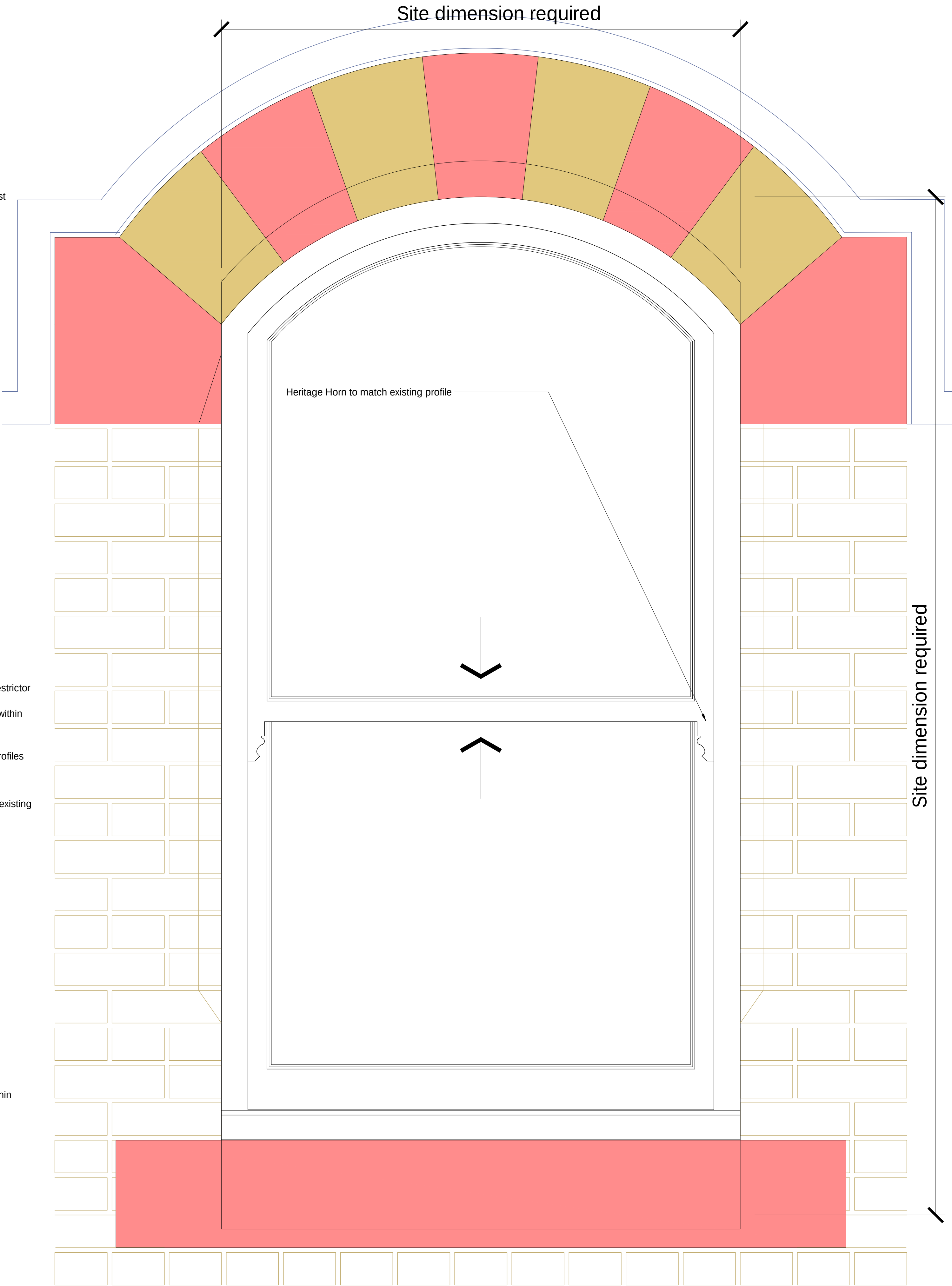
EXTERNAL ELEVATION
