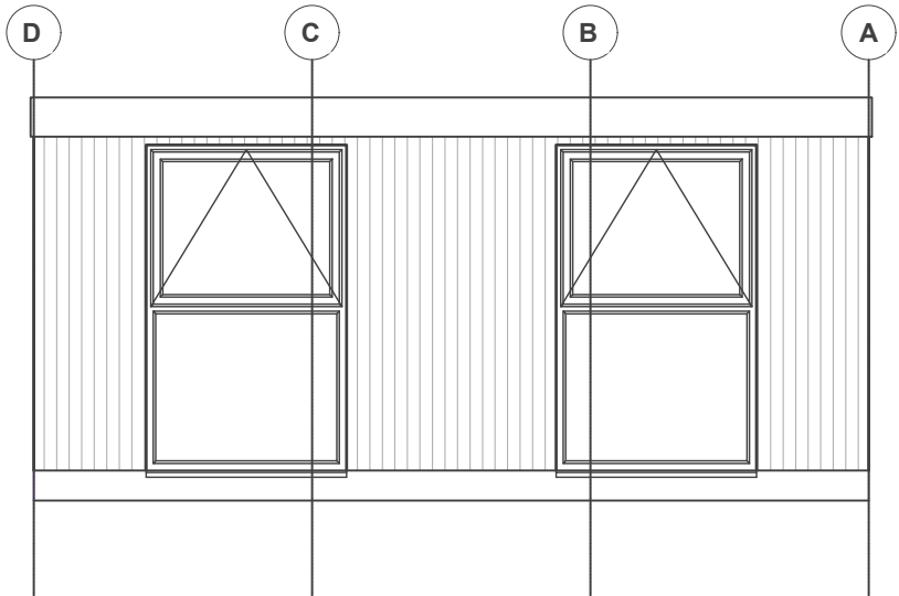
ELEVATION A FRONT 1:50
