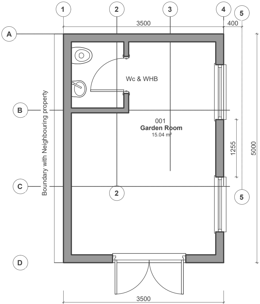
FLOOR PLAN 1:50
