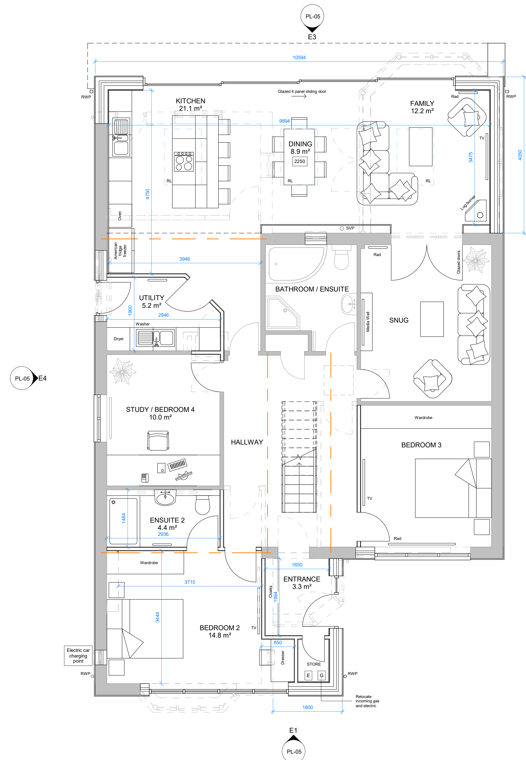
1 Proposed Ground Floor Level 1 : 50
