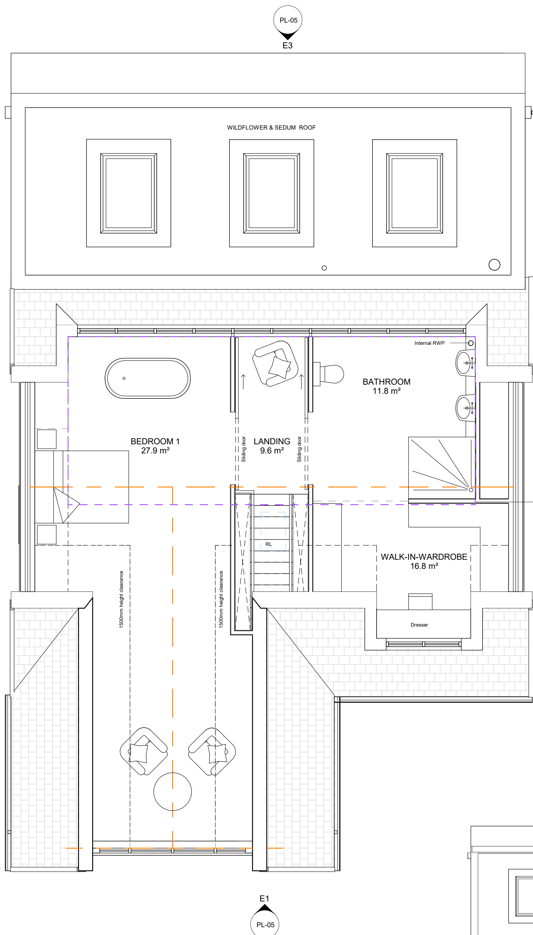
2 Proposed First Floor Level 1 : 50
