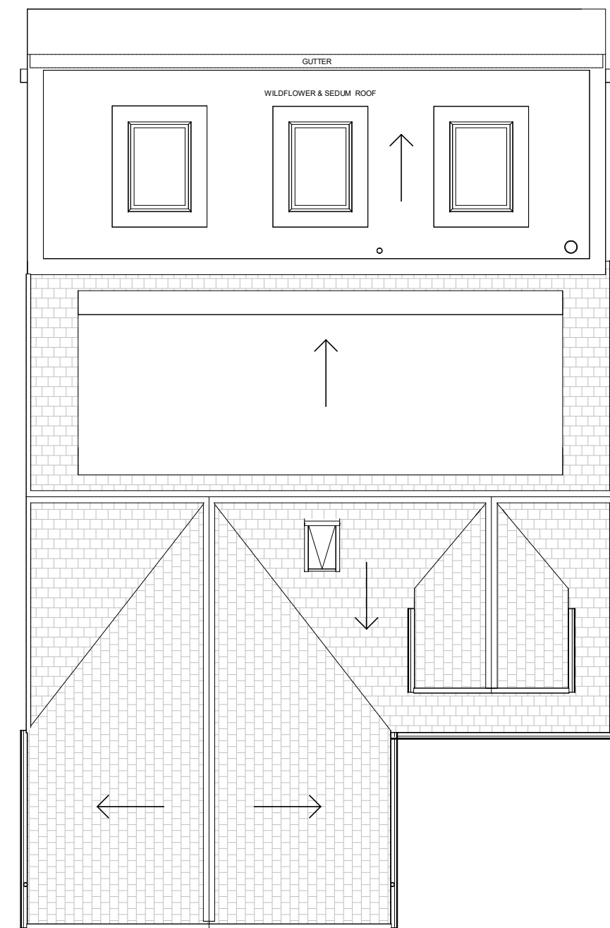
3 Proposed Roof Level 1 : 100
