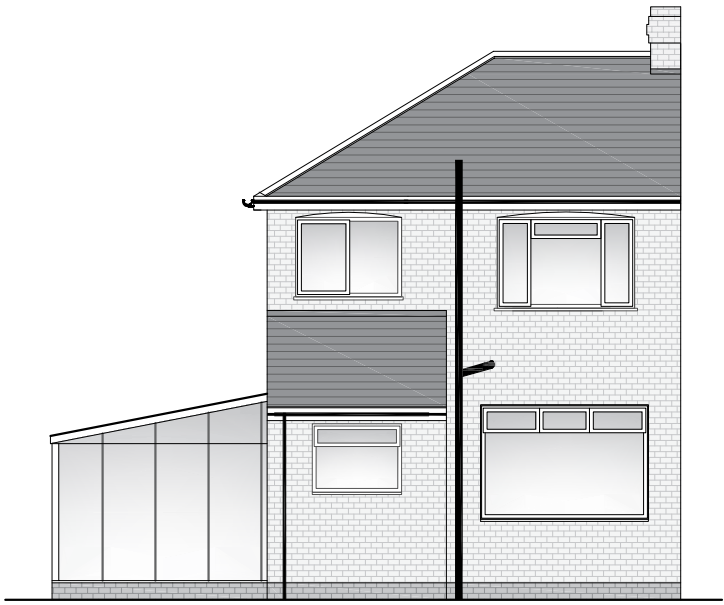
EXISTING REAR ELEVATION (Scale 1:100) SCALE BAR - (mm) 500 1000 2000
