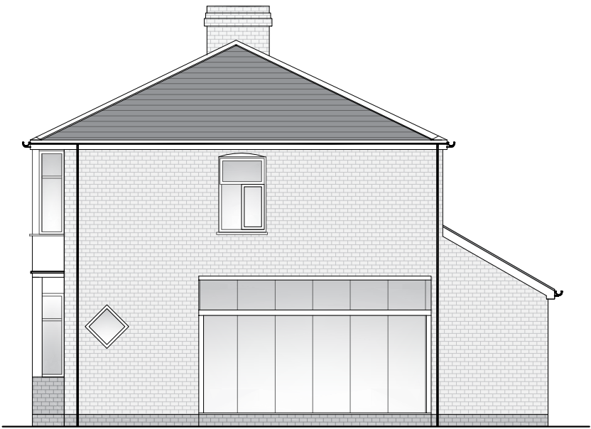
EXISTING SIDE ELEVATION (Scale 1:100) SCALE BAR - (mm) 500 1000 2000
