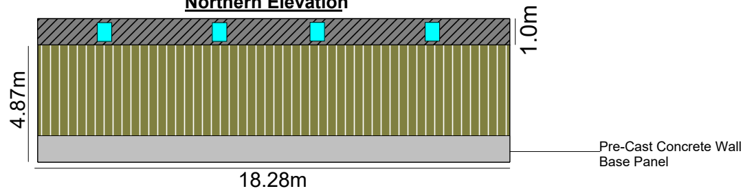
Northern Elevation
