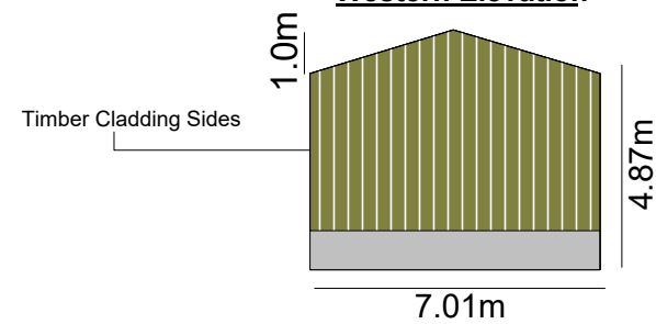
Western Elevation
