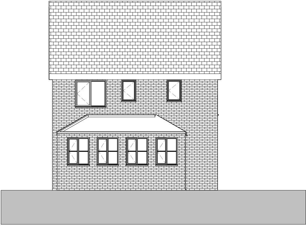
Rear Elevation 1 : 100
