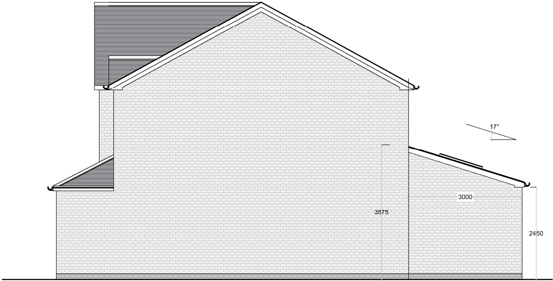
PROPOSED SIDE ELEVATION (Scale 1:100) SCALE BAR - (mm) 2000 1000 500
