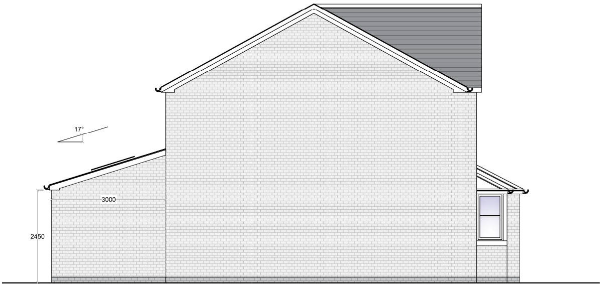
PROPOSED SIDE ELEVATION (Scale 1:100) SCALE BAR - (mm) 500 1000 2000
