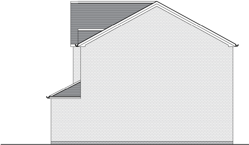
EXISTING SIDE ELEVATION (Scale 1:100) SCALE BAR - (mm) 2000 1000 500
