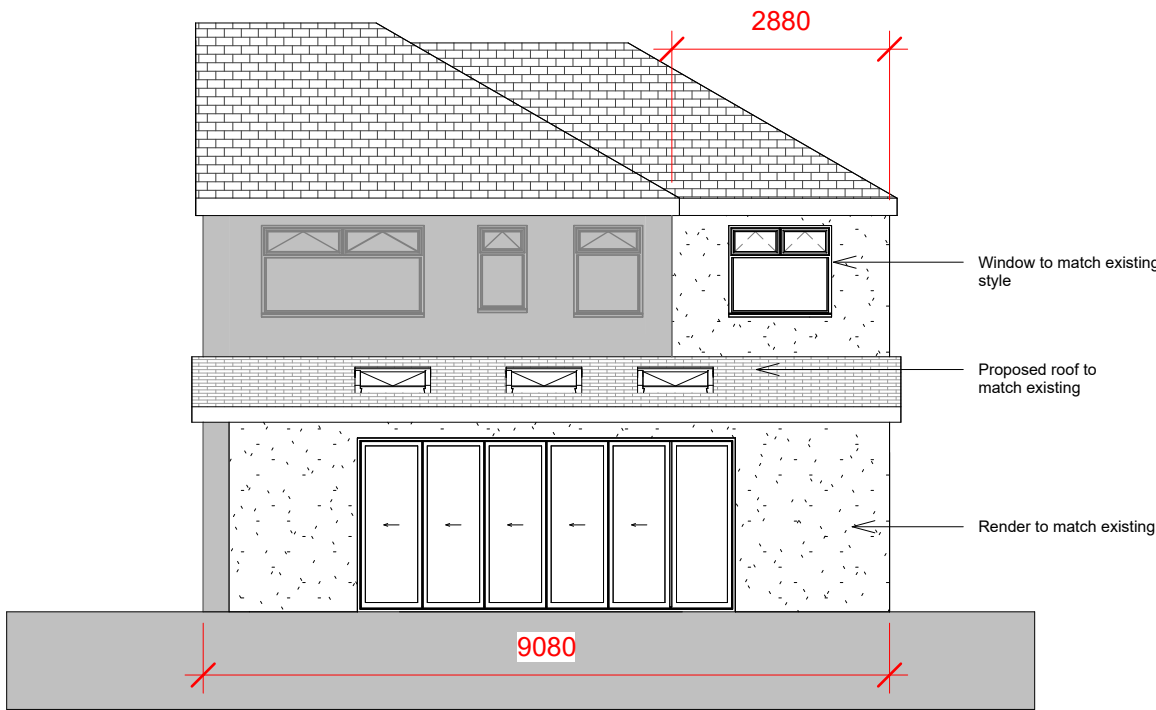
Rear Elevation 1 : 100
