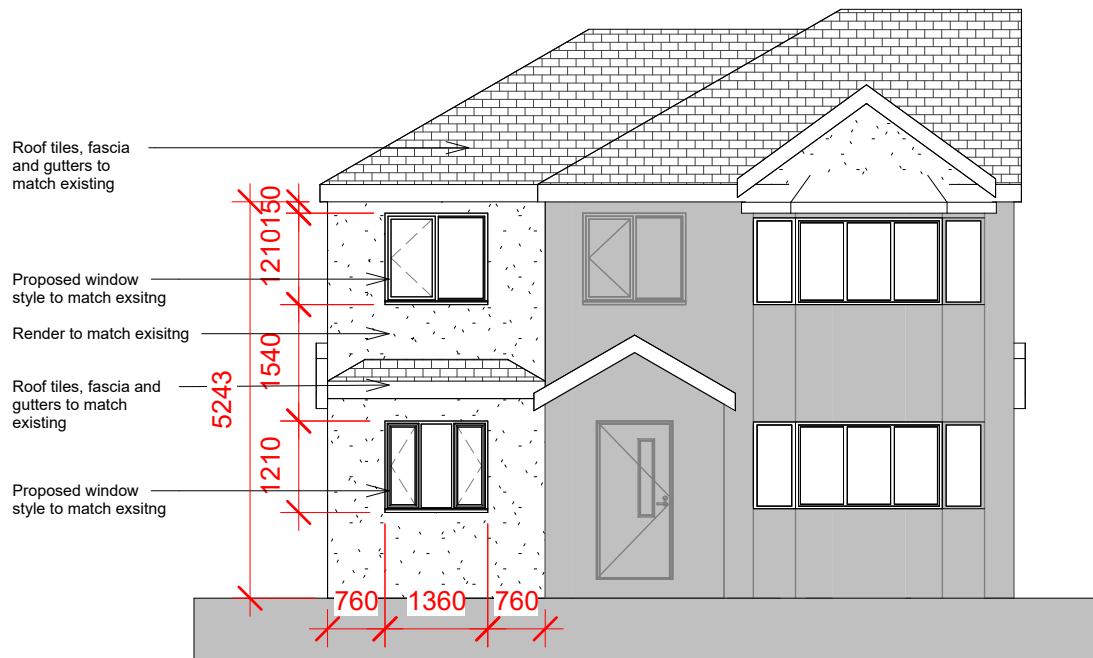
Front Elevation 1 : 100
