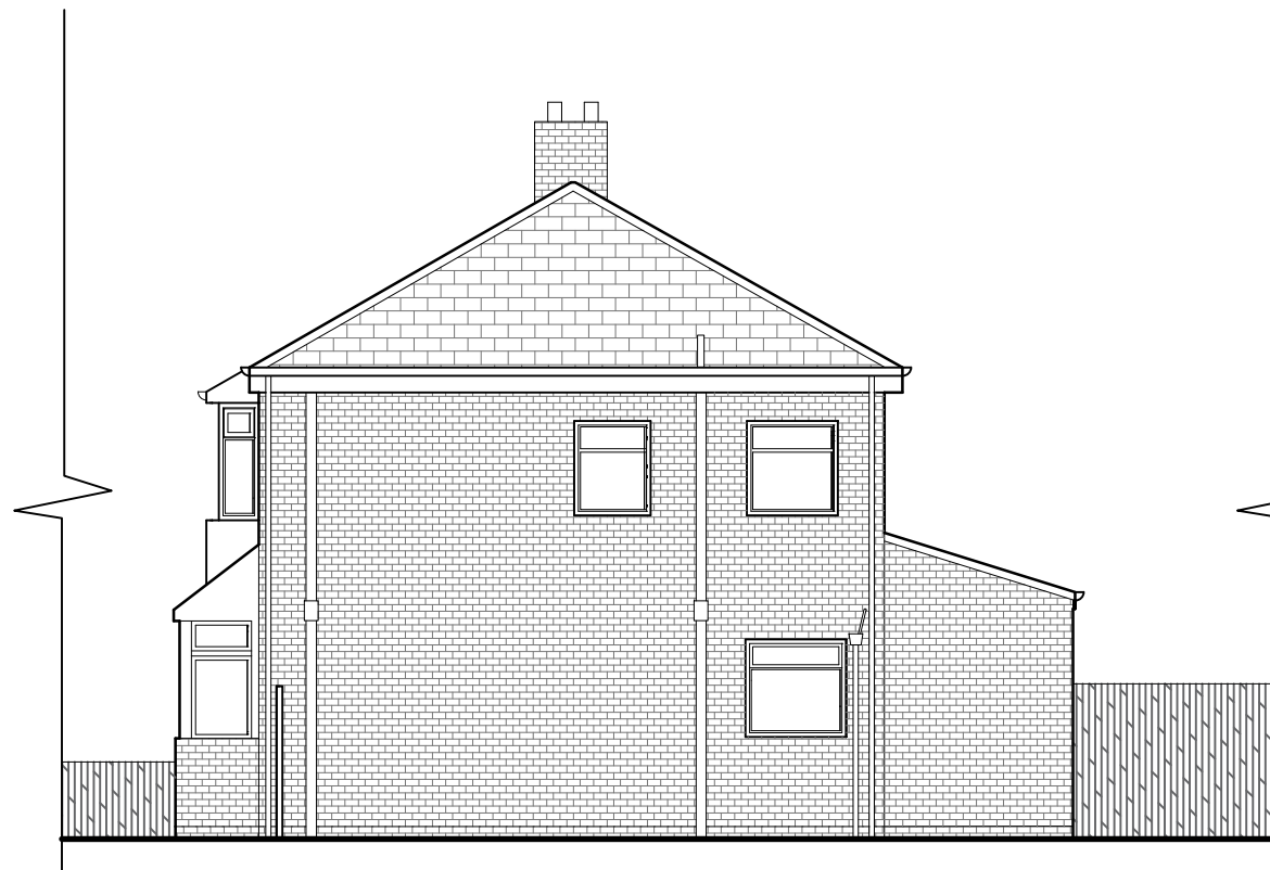
EXISTING ELEVATION B-B SCALE 1:100
