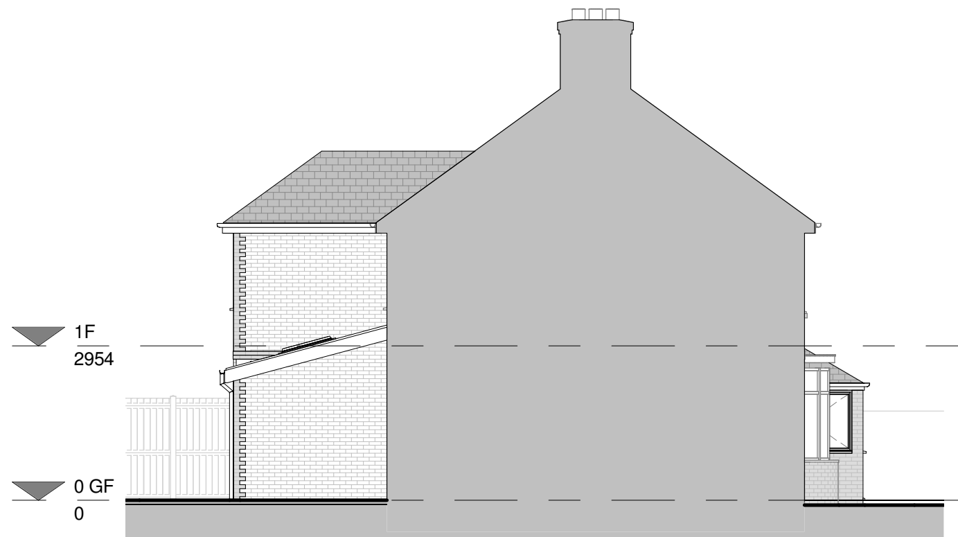
SIDE ELEVATION II
