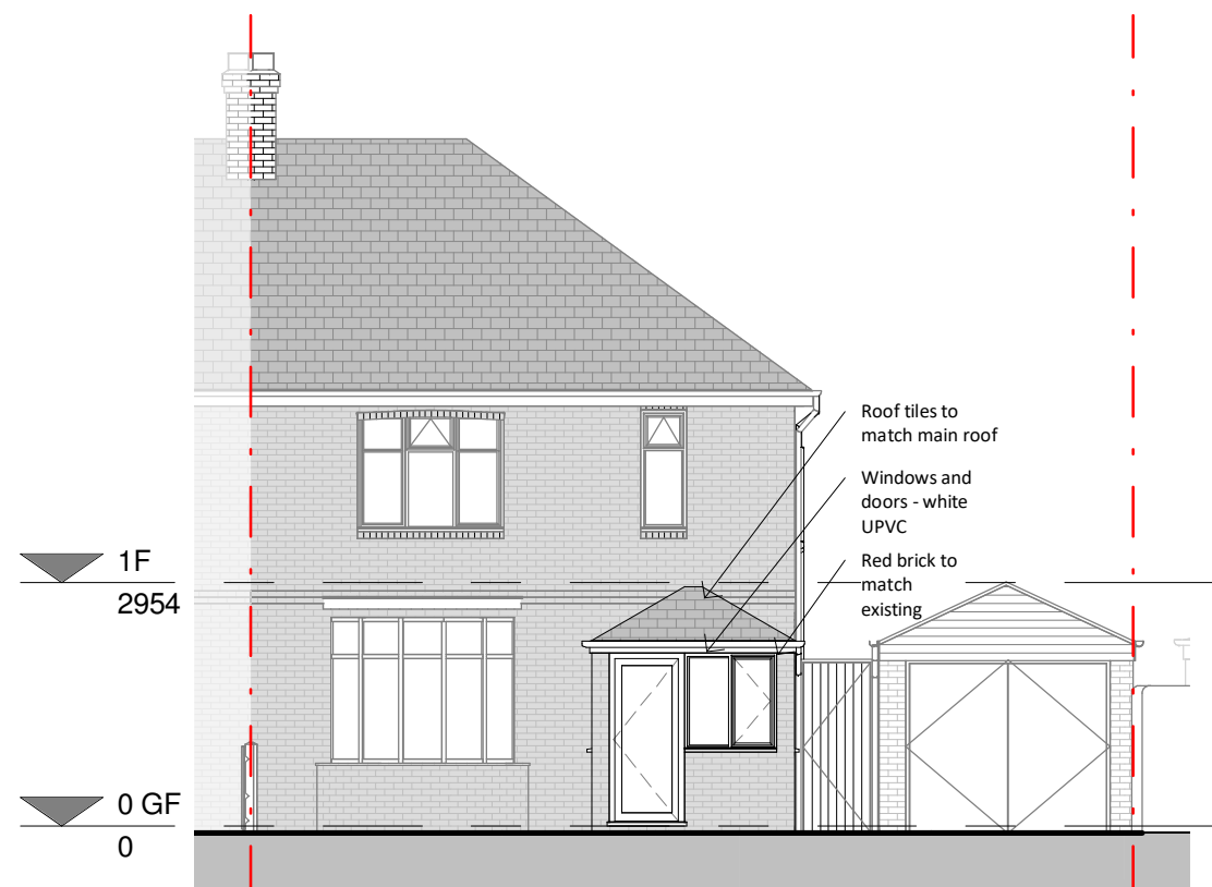
FRONT ELEVATION
