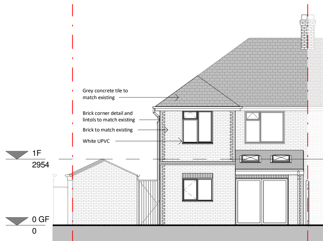
REAR ELEVATION
