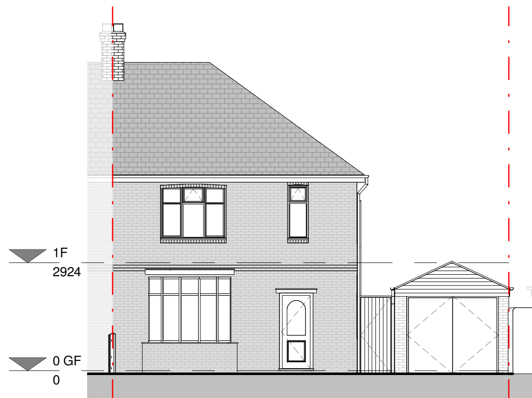
FRONT ELEVATION
