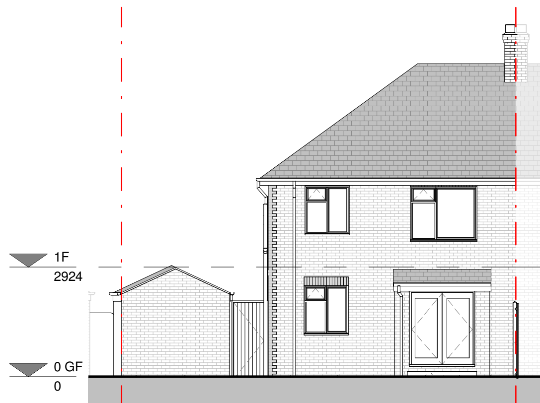
REAR ELEVATION
