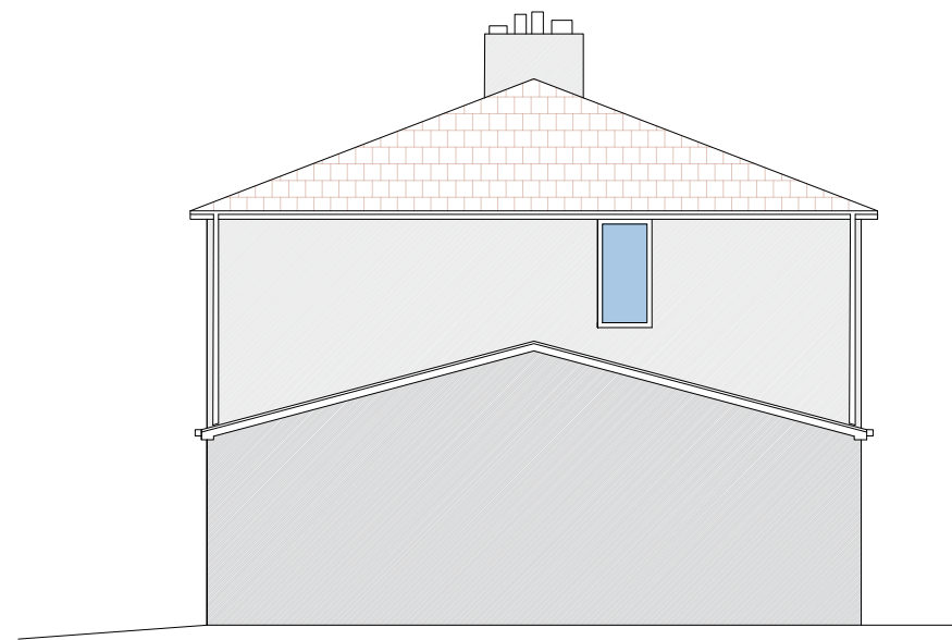
EXISTING RIGHT-HAND SIDE ELEVATION
