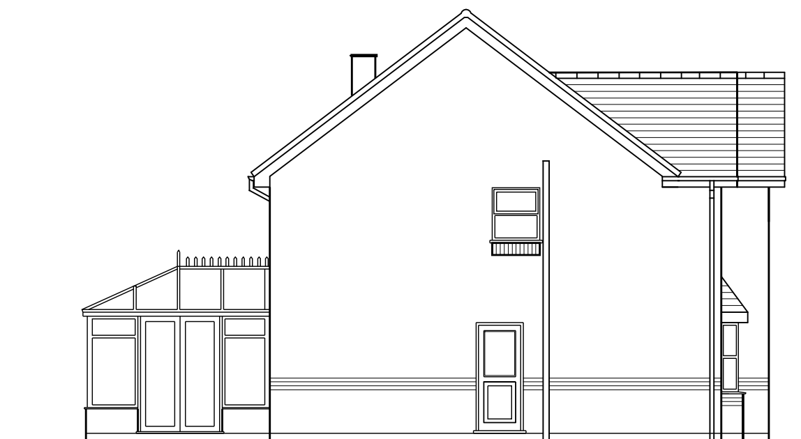
Existing Side Elevation. East Facing
