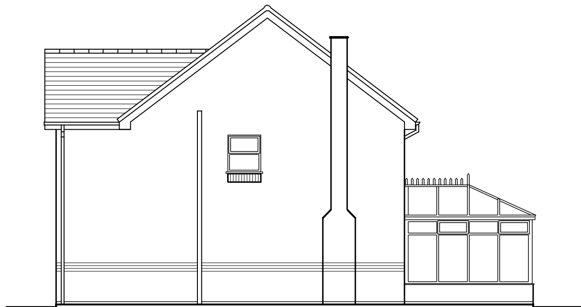
Existing Side Elevation. West Facing
