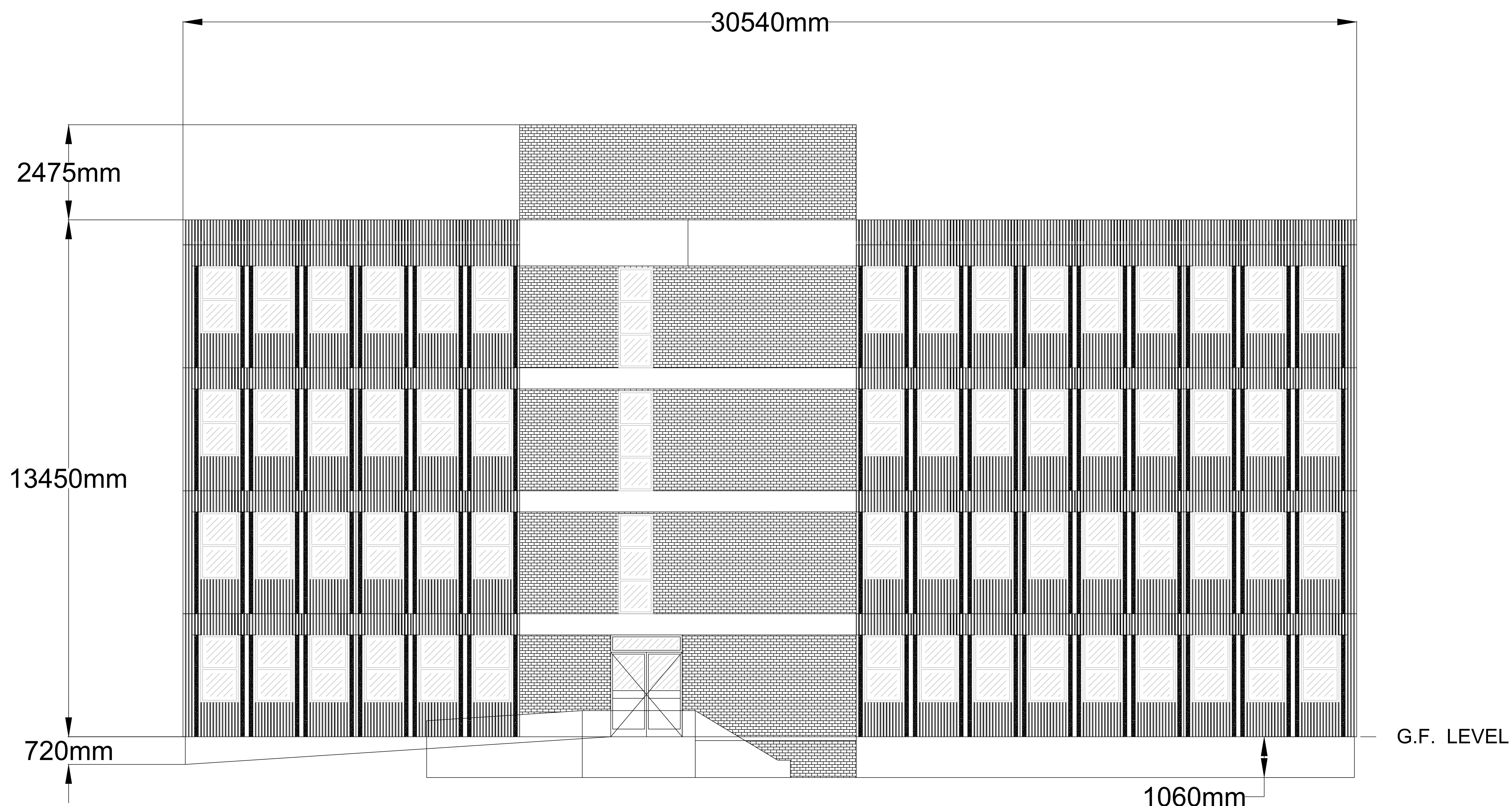
Rear Elevation C - Multi-Storey Car Park Side
