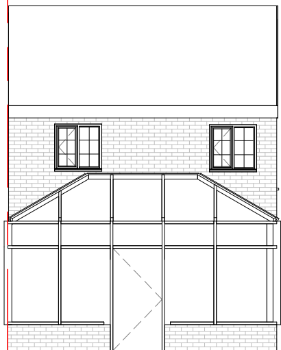
Exist. Rear Elevation 1 : 100
