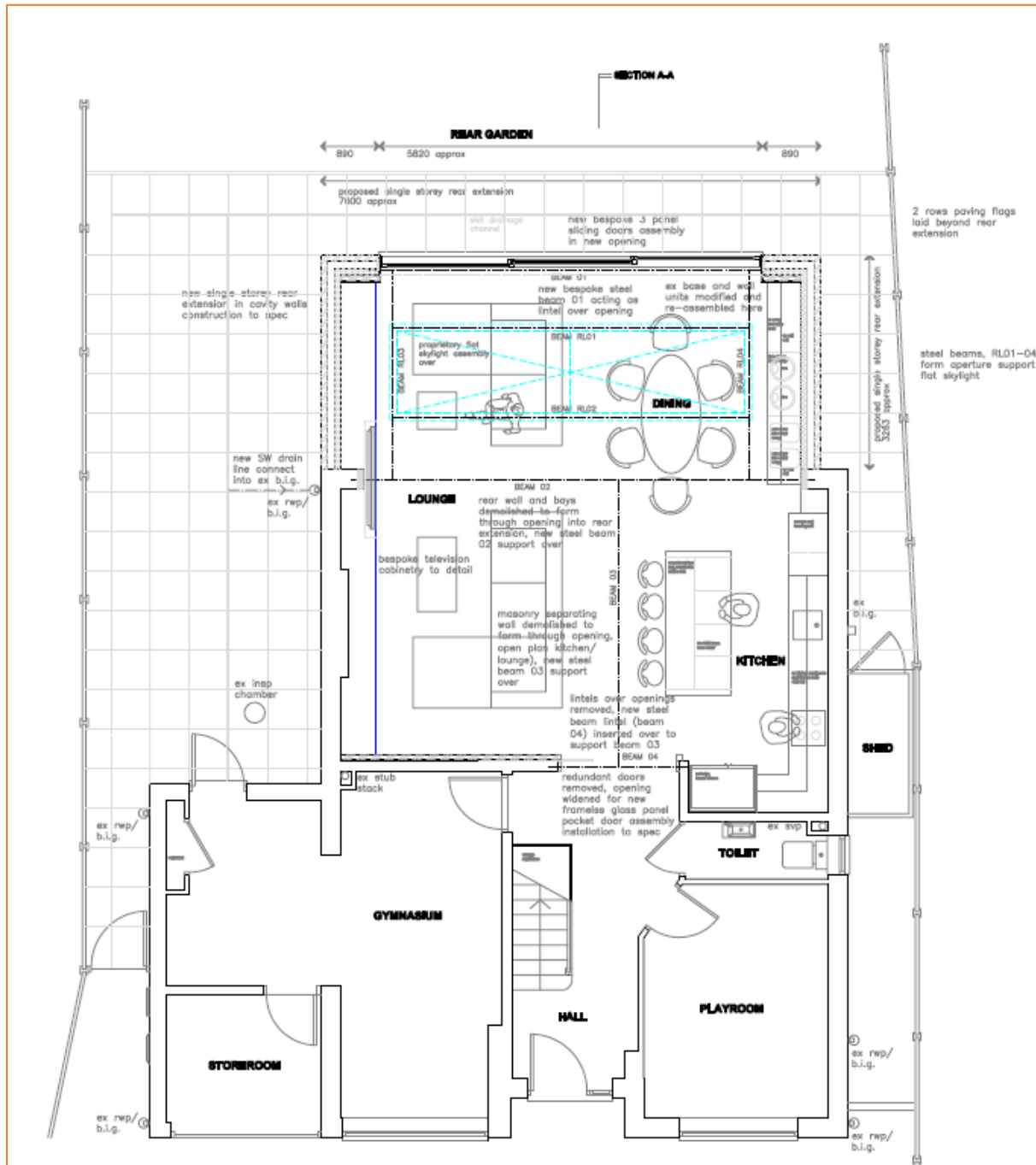
Figure 5: Proposed development plans (Source: Team2Design)
