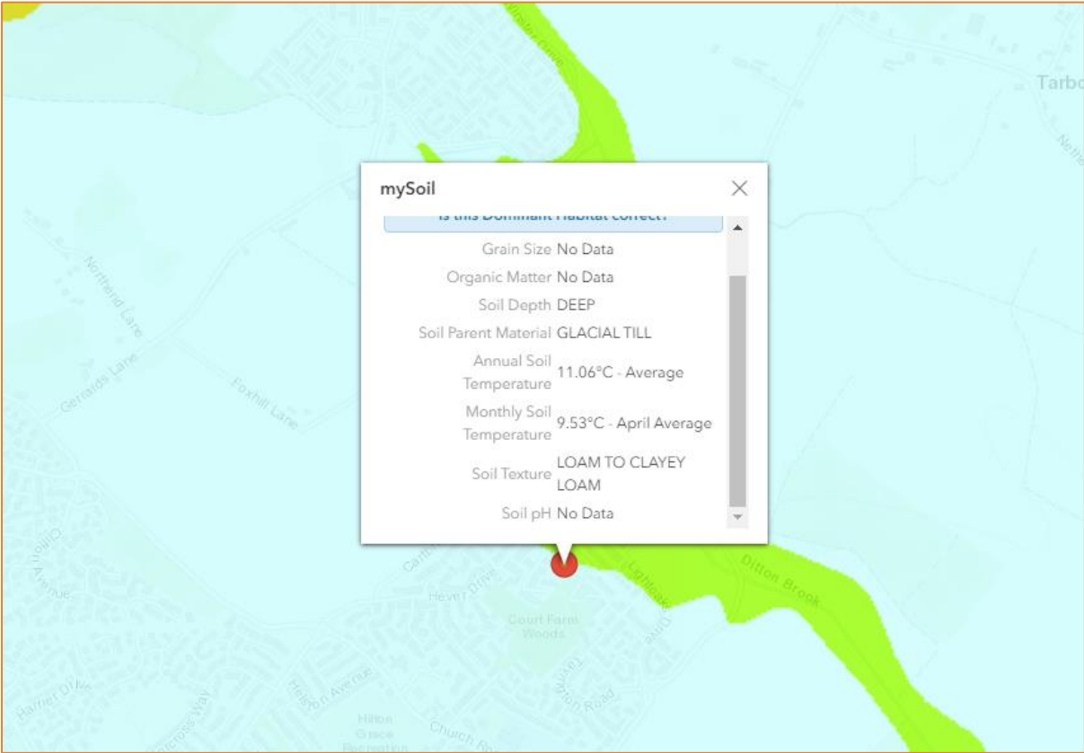
Figure 4: Local soil types (Source: UKSO)
