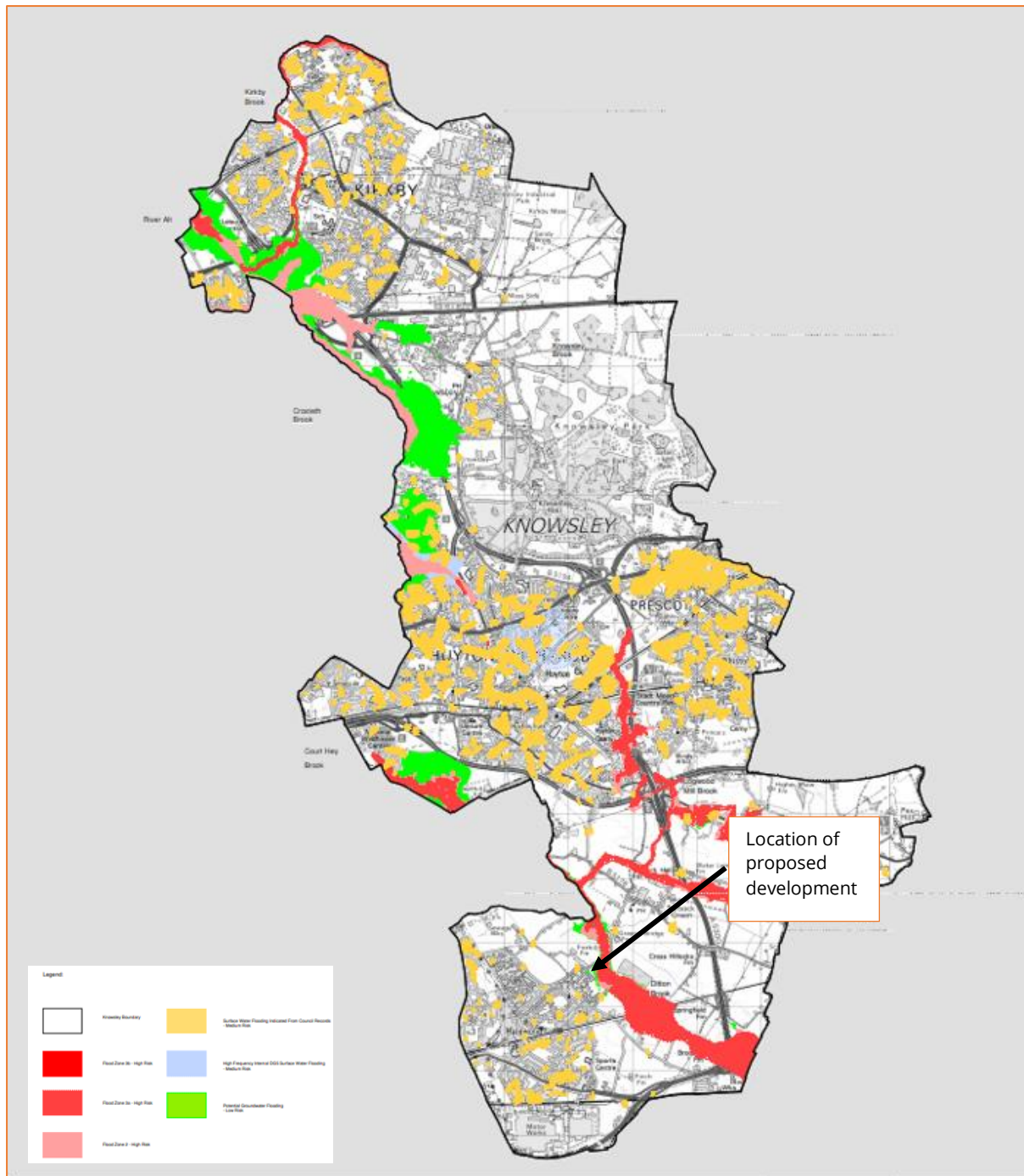
Figure 7: Combined Risk Matrix Map (Source: Knowsley and Sefton Council Strategic Flood Risk Assessment 2009)
