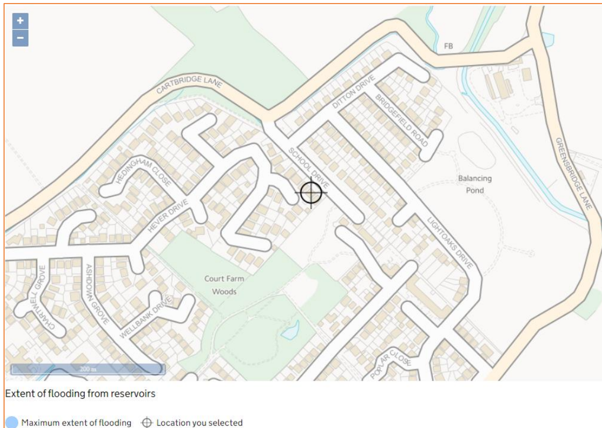
Figure 9: Extract from Environment Agency Risk of Flooding from Reservoirs Map (Source: EA)
