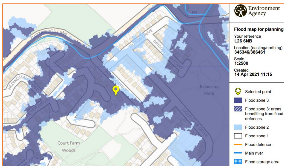
Figure 6: Environment Agency Flood Map for Planning (Rivers and Sea) (Source: EA)
