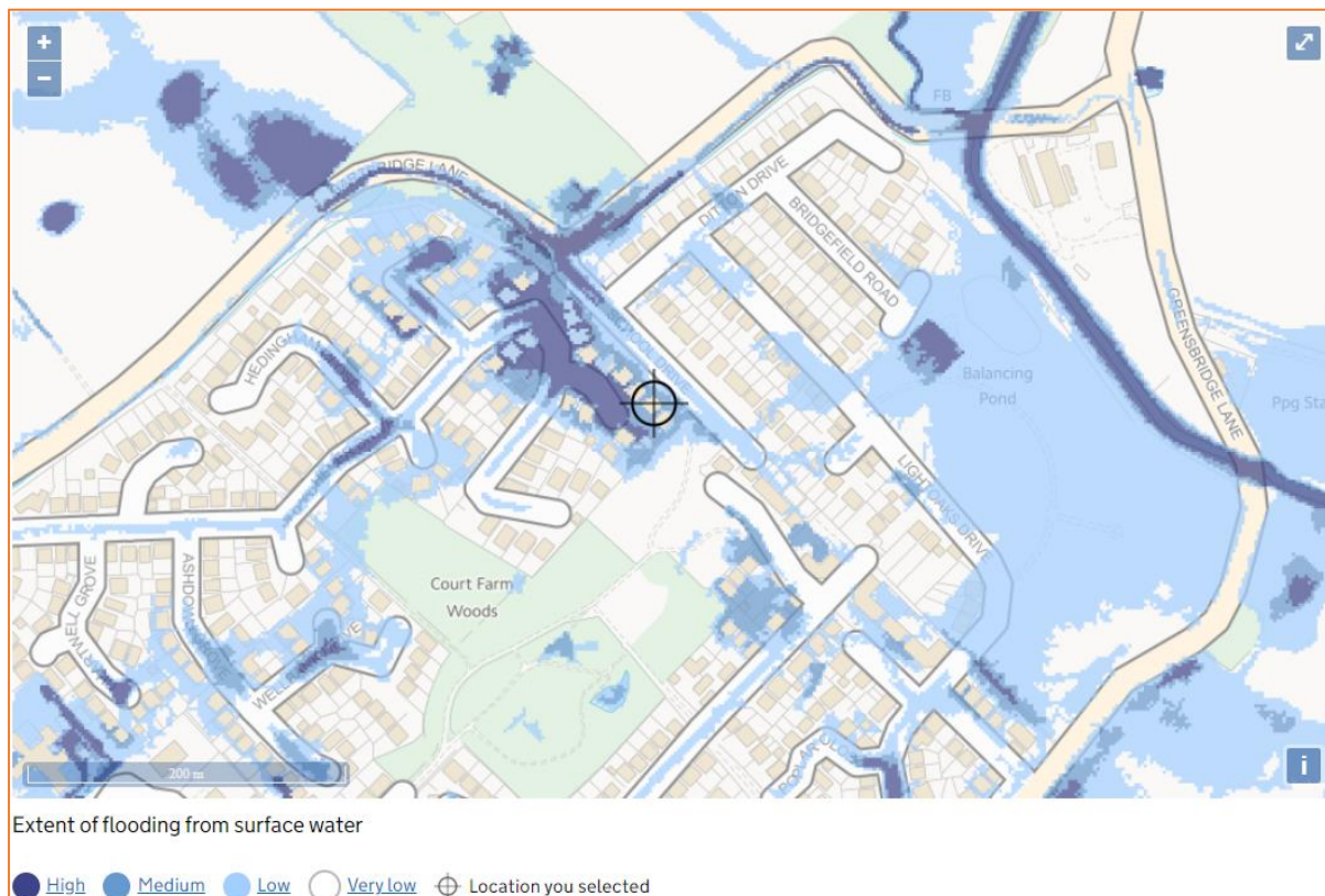
Figure 8: Extract from Environment Agency Surface Water Flood Map (Source: EA)
