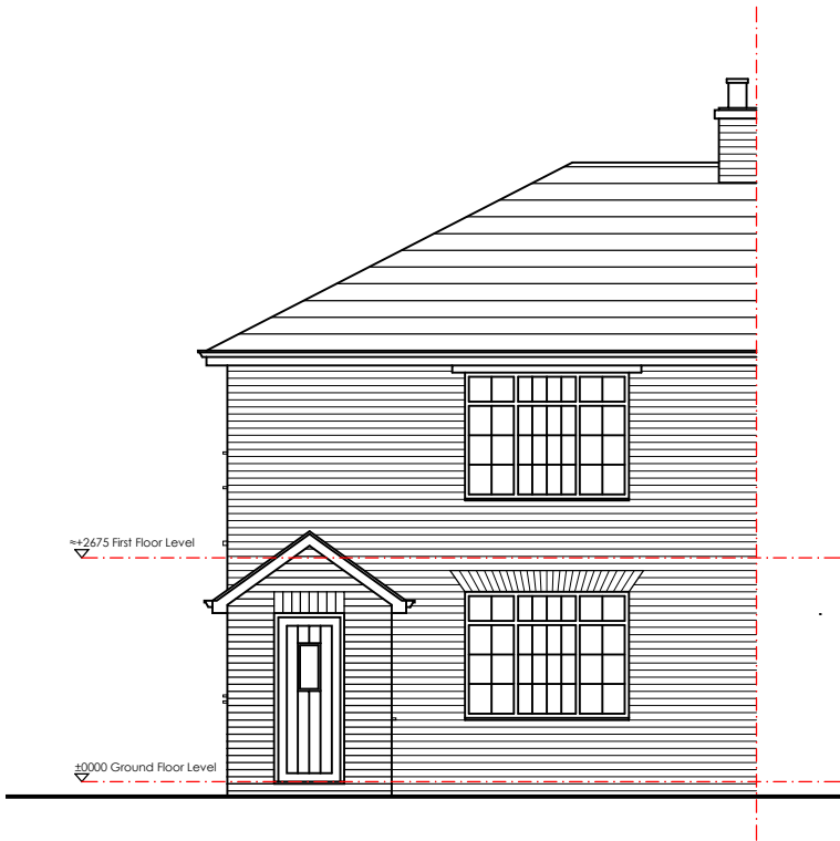
Front Elevation
