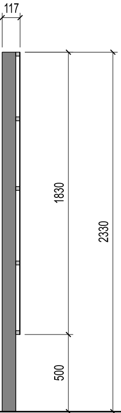
SIDE ELEVATION
