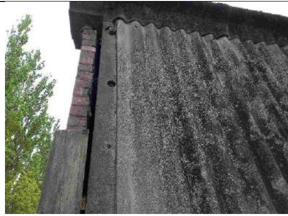
Photograph 14: Gaps present between adjoining walls on north-eastern corner of B2
