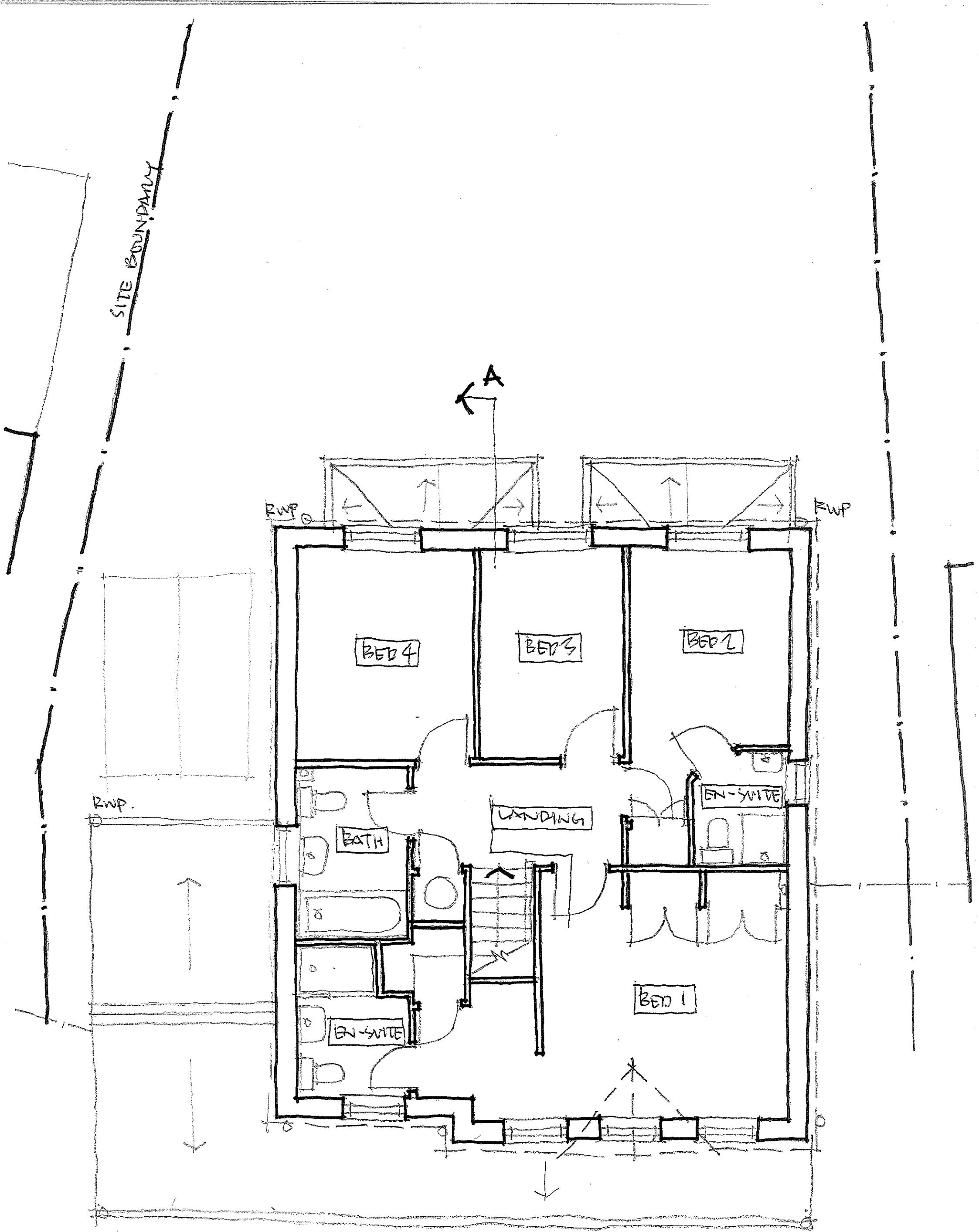
E03. EXISTING FIRST FLOOR PLAN 1:50 ← A PROPOSED EXTENSION TO 55 HEVER DRIVE L26 6LN
