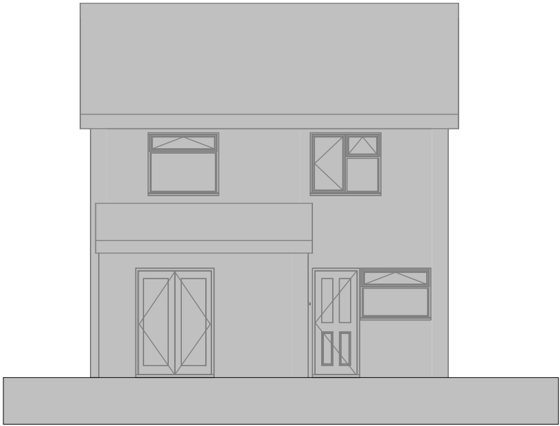
Rear Elevation 1 : 100
