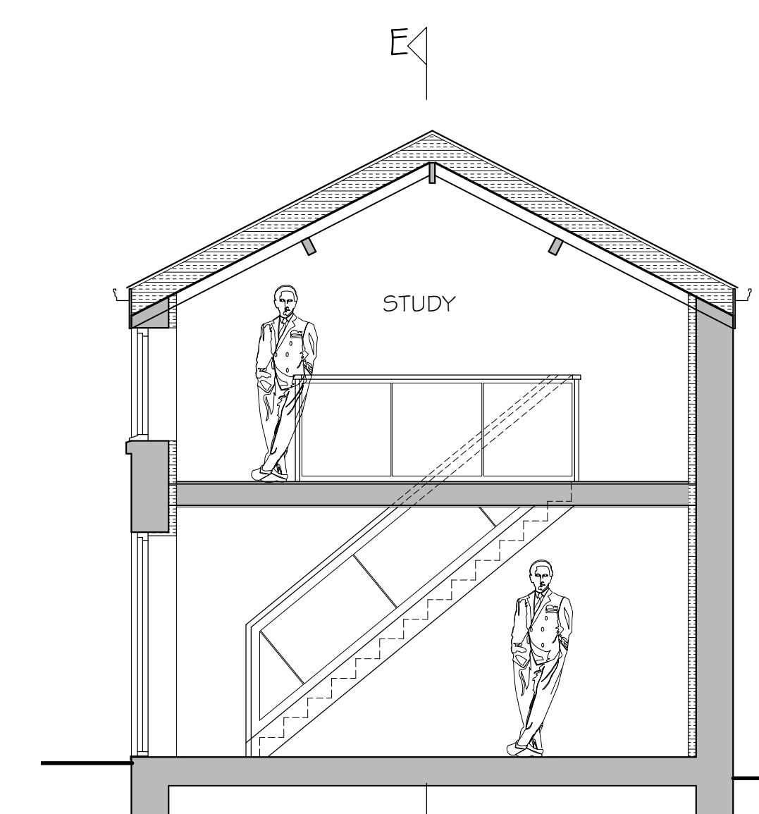
PROPOSED SECTION G-G (1:50)
