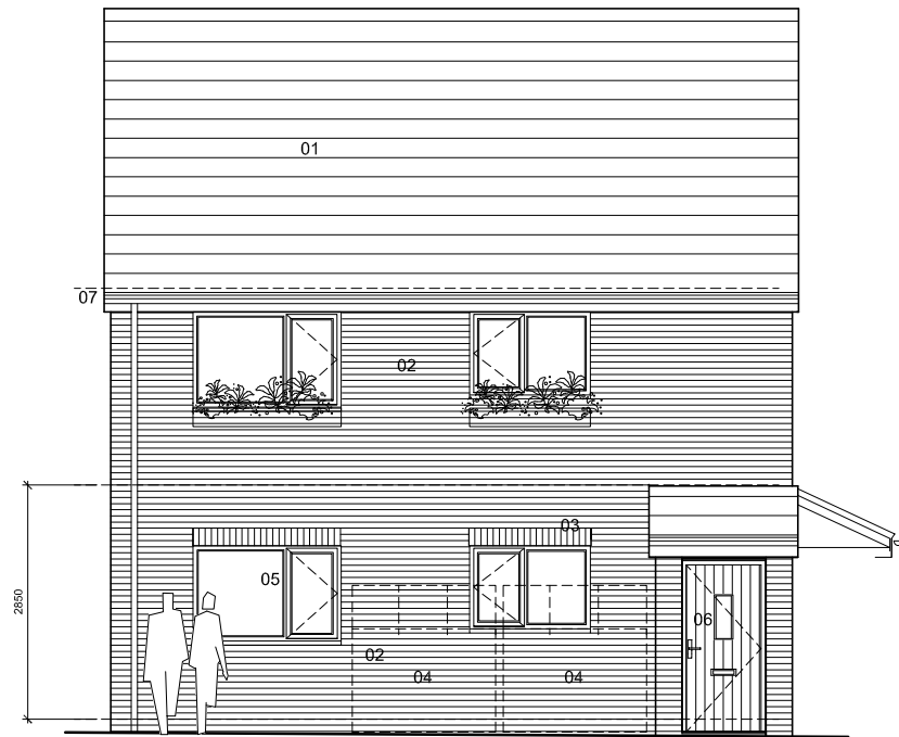
south elevation
