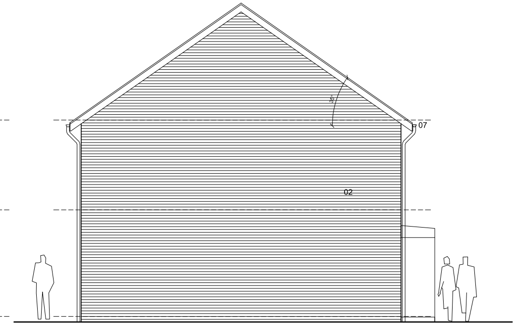
side elevations
