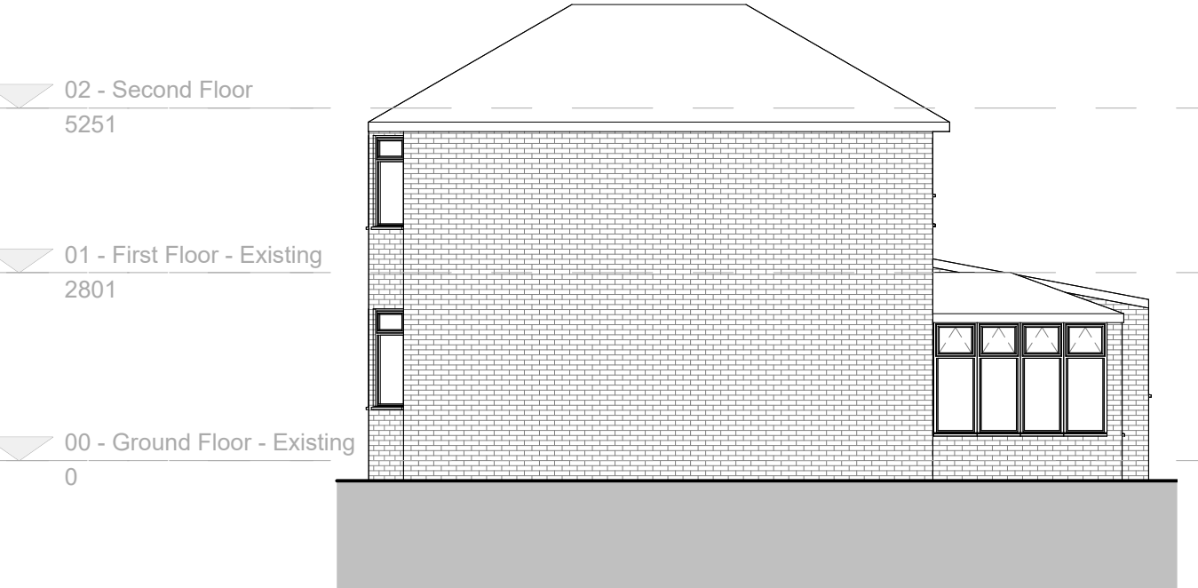
Right Side Elevation - Existing
