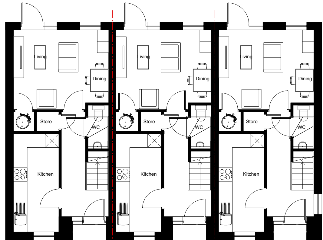
Ground Floor
