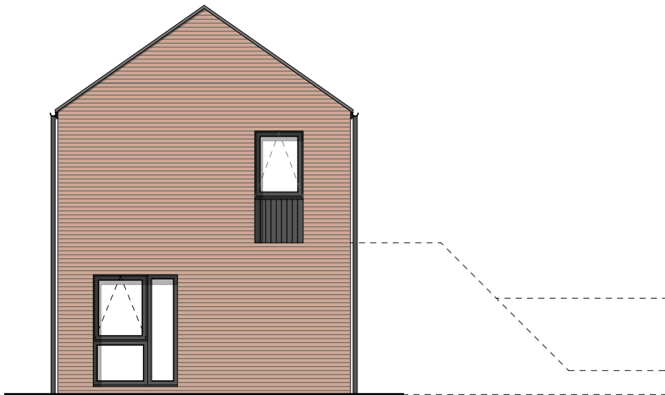
Side Elevation
