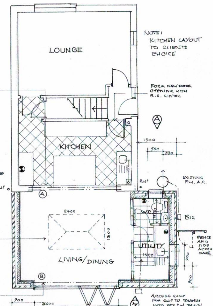
GROUND FLOOR PLAN 1:50
