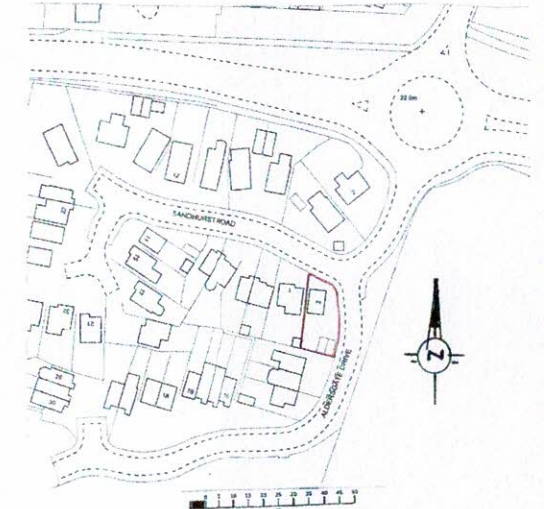
LOCATION PLAN 1:1250
