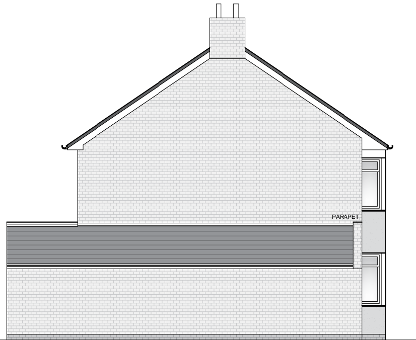
EXISTING SIDE ELEVATION (Scale 1:100) SCALE BAR - (mm) 500 1000 2000
