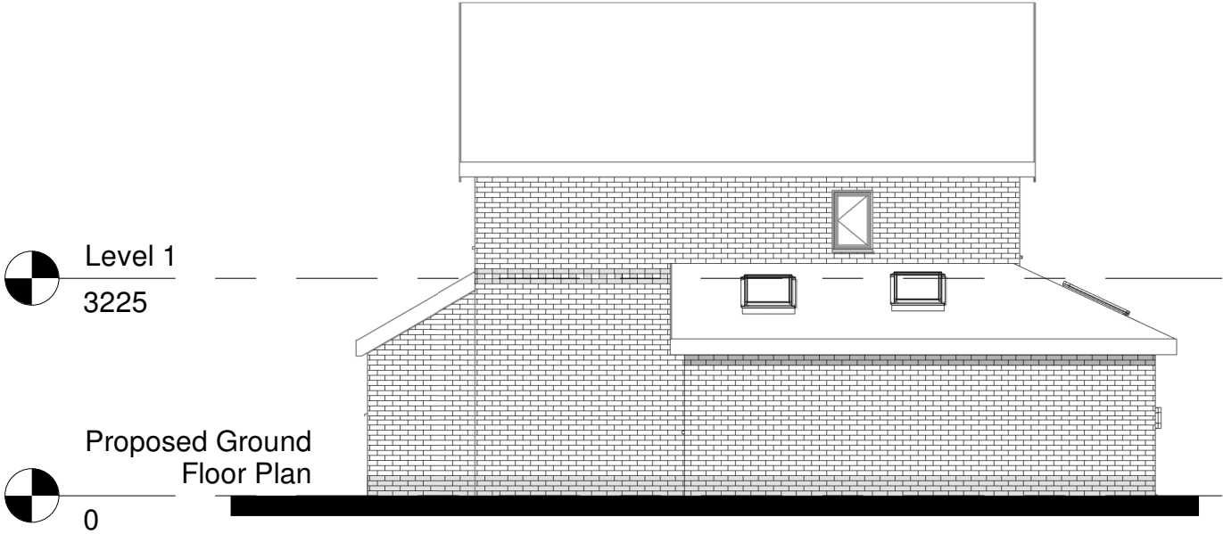
Prop. Gable Elevation 1 : 100
