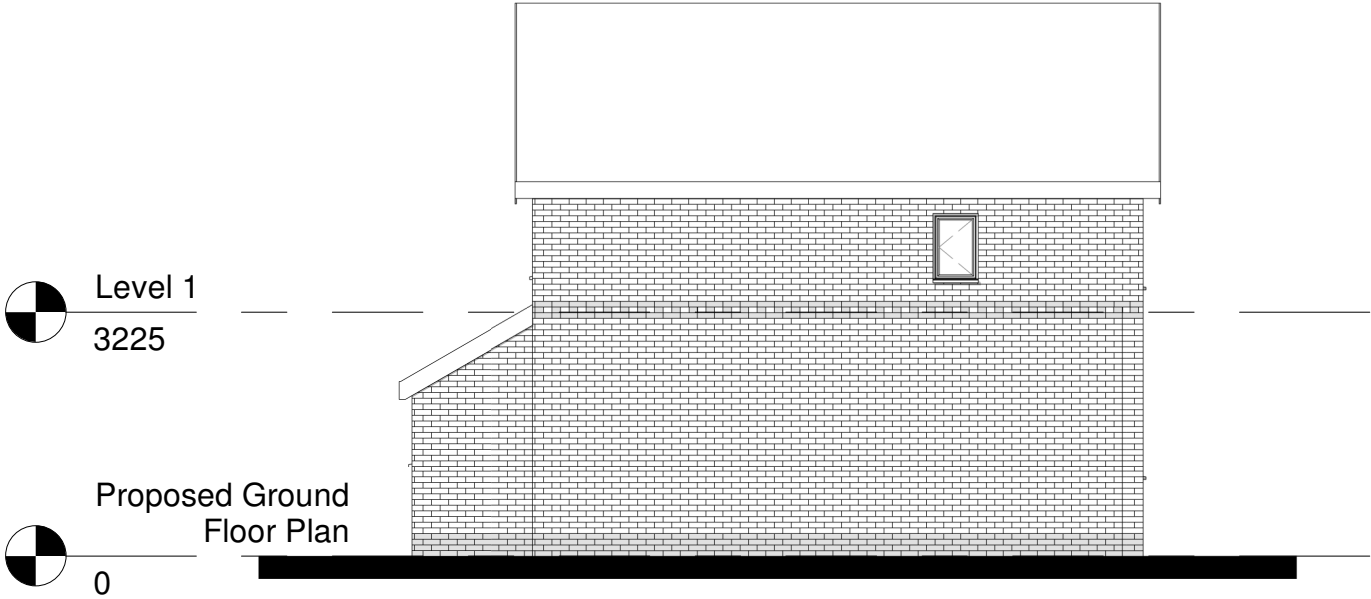
Exist. Gable Elevation 1 : 100
