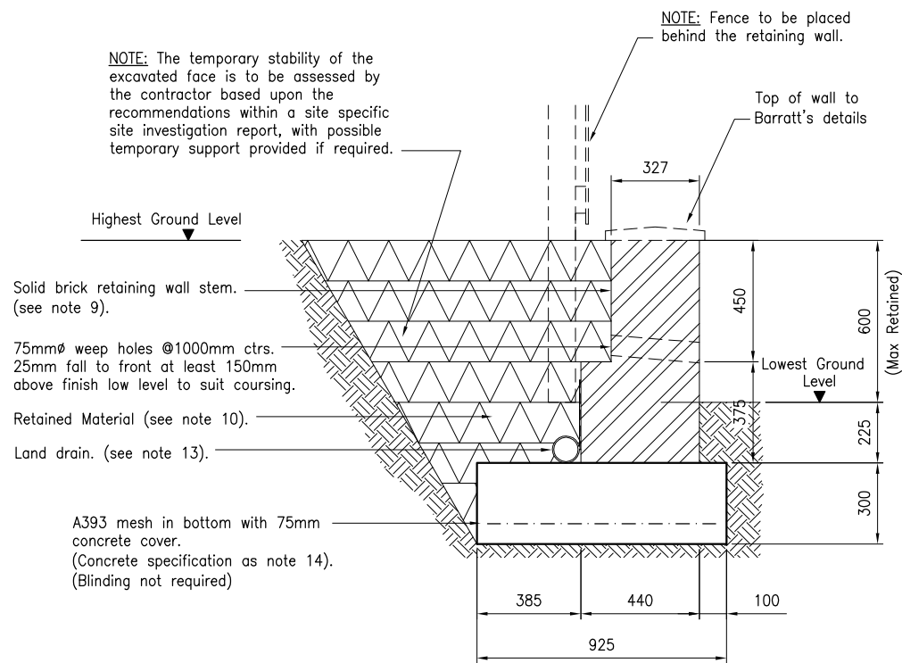
SECTION THRO' SOLID BRICK RETAINING WALL (600 RETAINED) (SCALE @ 1:25)
