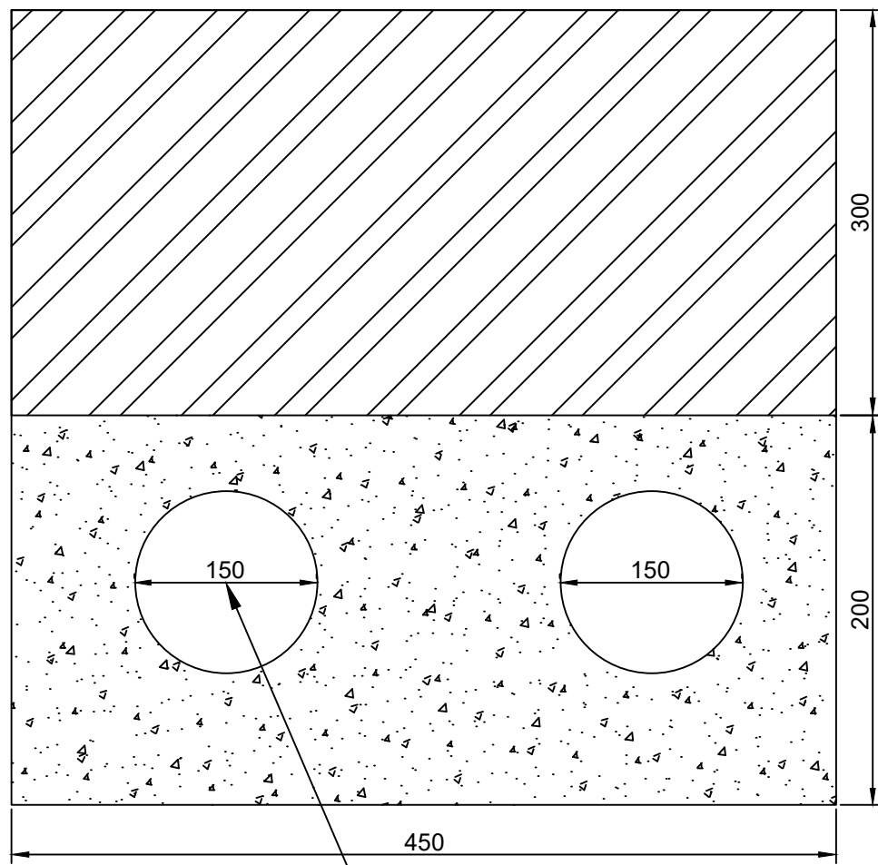
TYPE 3 MOT TWIN 1500 PREMORE PIPE
