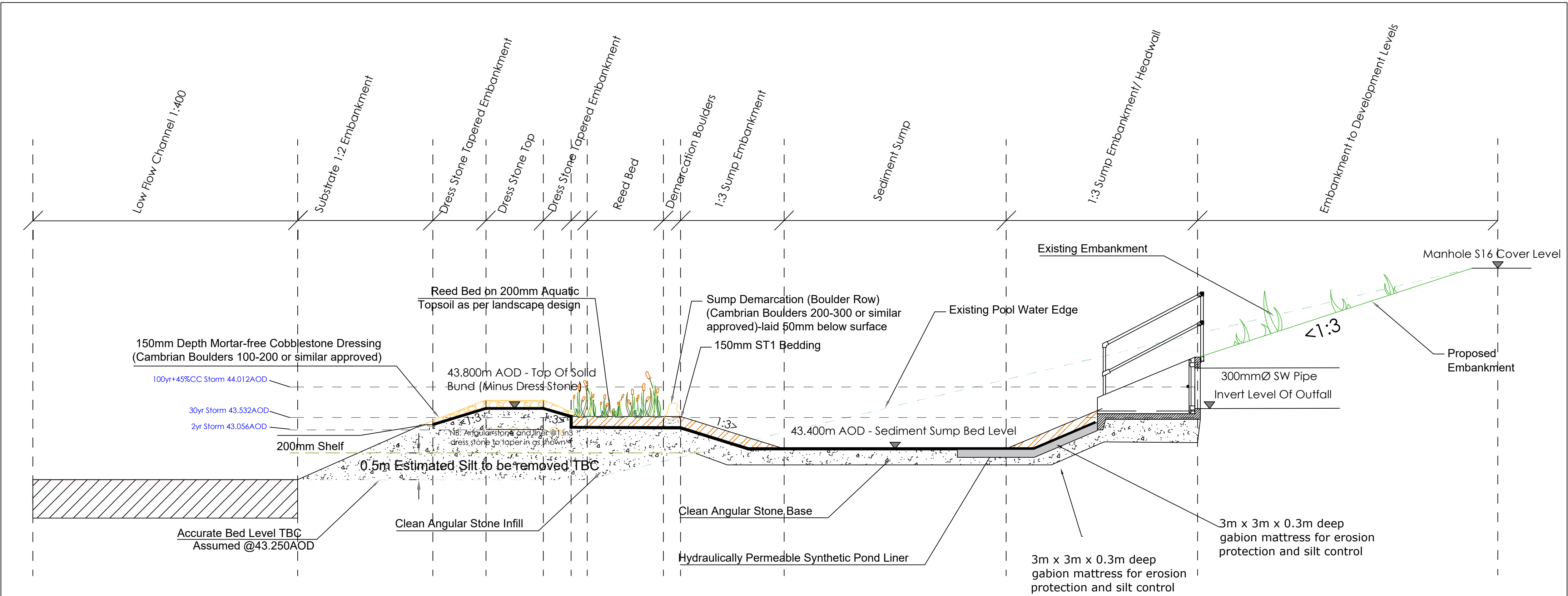
Sediment Forebay Basin 8.002 X-Sect A-A Scale 1:50
