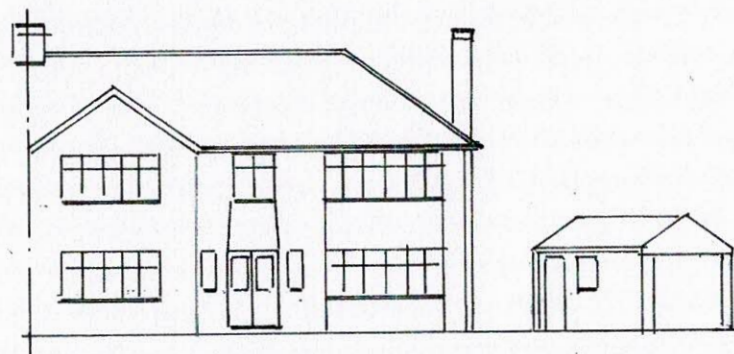
FRONT ELEVATION 1:100
