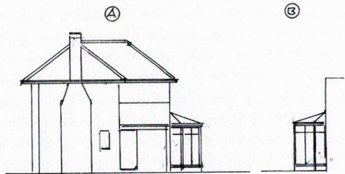
SIDE ELEVATIONS 1:100
