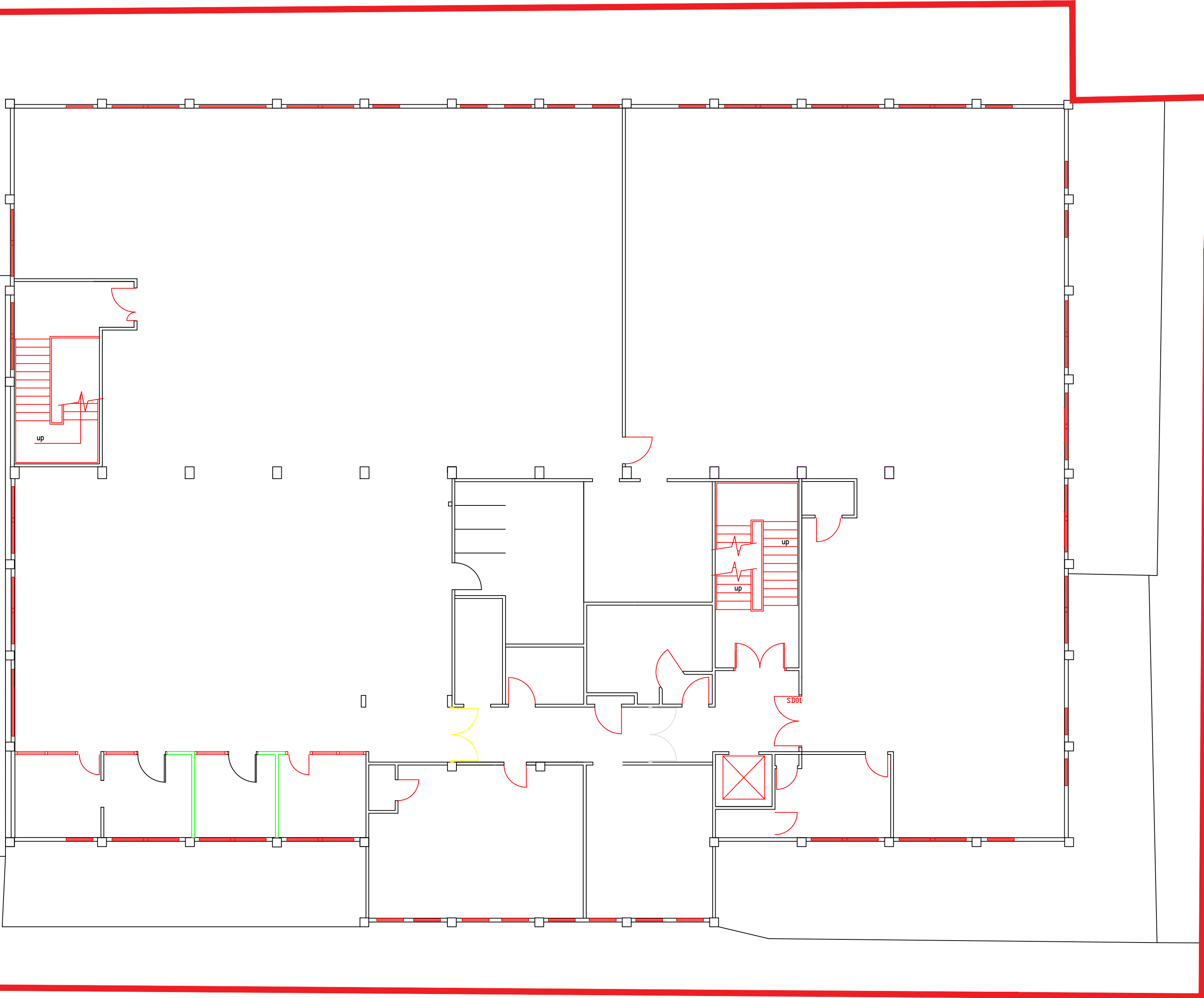
EXISTING SECOND FLOOR PLAN
