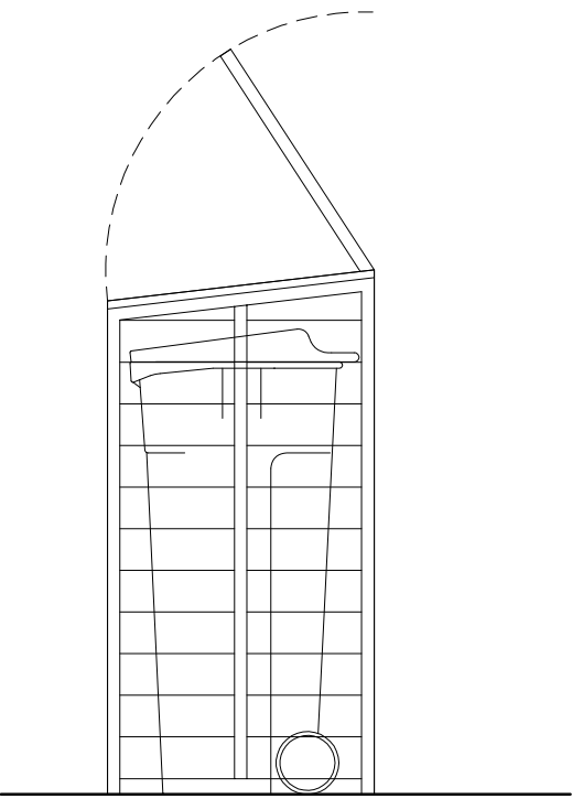
SIDE ELEVATION
