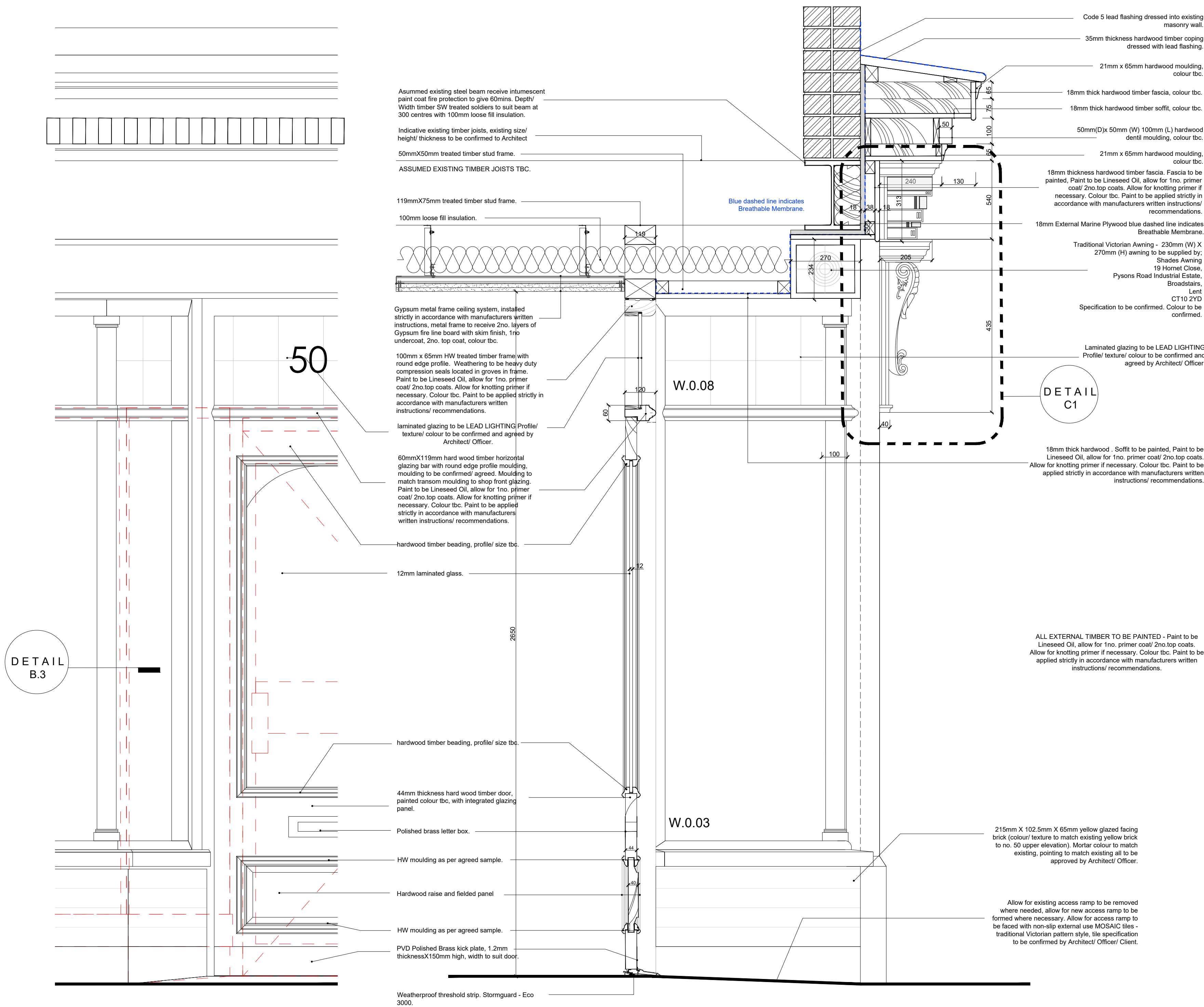
Proposed Shop Front Part Elevation Scale 1:10
