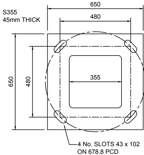
FLANGE PLATE DETAIL
