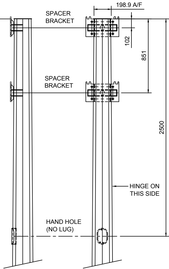
COLUMN TOP DETAIL
