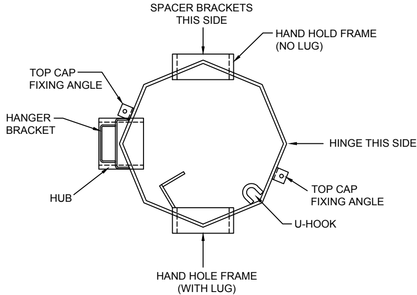
INDICATIVE PLAN SHOWING ORIENTATION OF ATTACHMENTS
