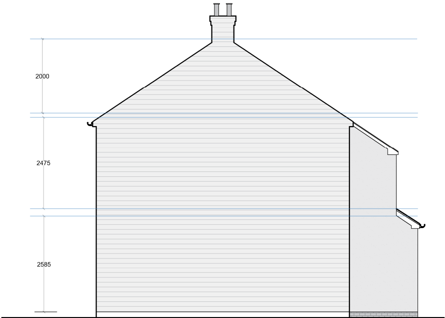
EXISTING SIDE ELEVATION (Scale 1:100) SCALE BAR - (mm) 2000 1000 500
