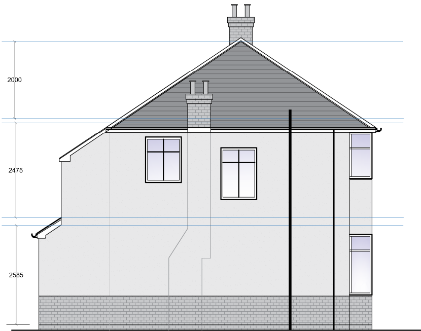
EXISTING SIDE ELEVATION (Scale 1:100) SCALE BAR - (mm) 500 1000 2000
