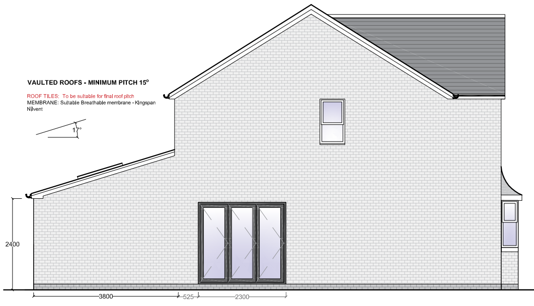
PROPOSED SIDE ELEVATION (Scale 1:100) SCALE BAR - (mm) 500 1000 2000
