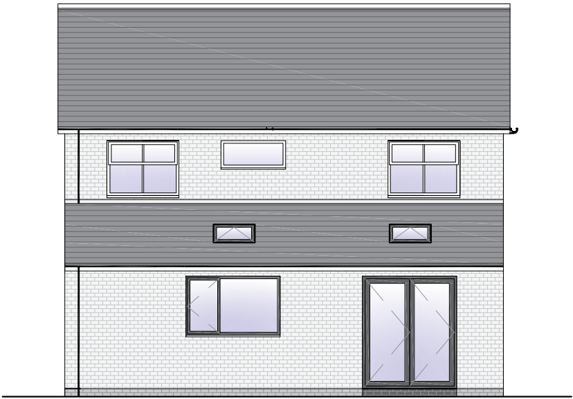
PROPOSED REAR ELEVATION (Scale 1:100) SCALE BAR - (mm) 500 1000 2000
