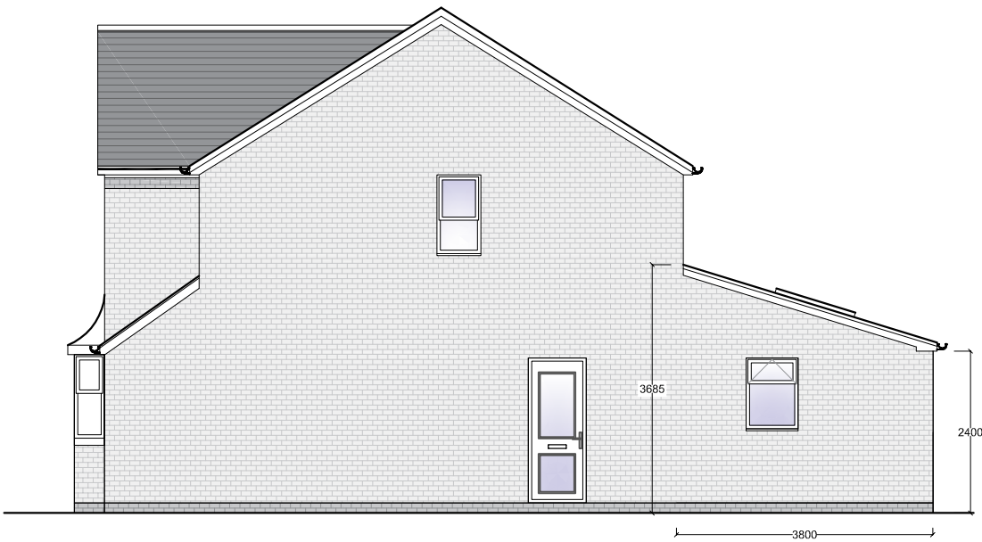
PROPOSED SIDE ELEVATION (Scale 1:100) SCALE BAR - (mm) 500 1000 2000
