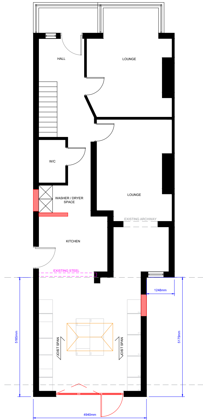
GROUND FLOOR
