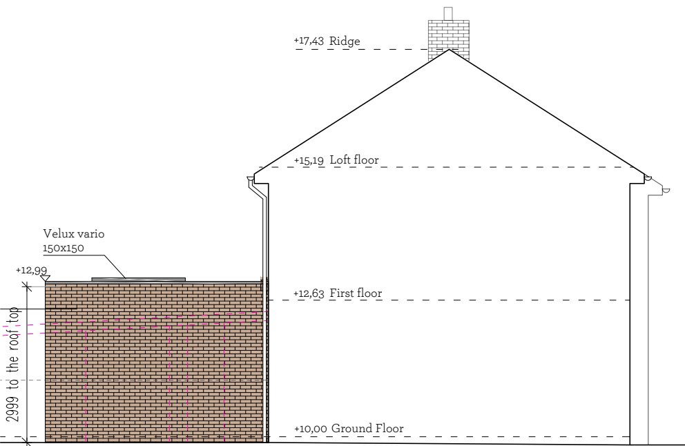
Side Elevation 2
